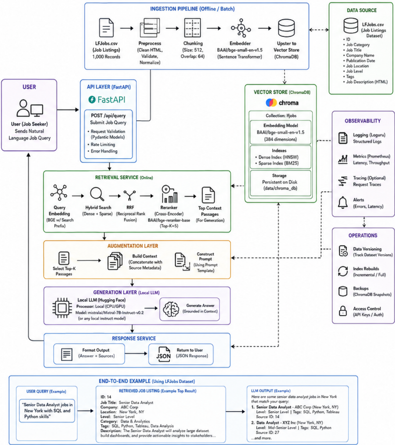
Figure 10: High-Level Architecture of the RAG System
